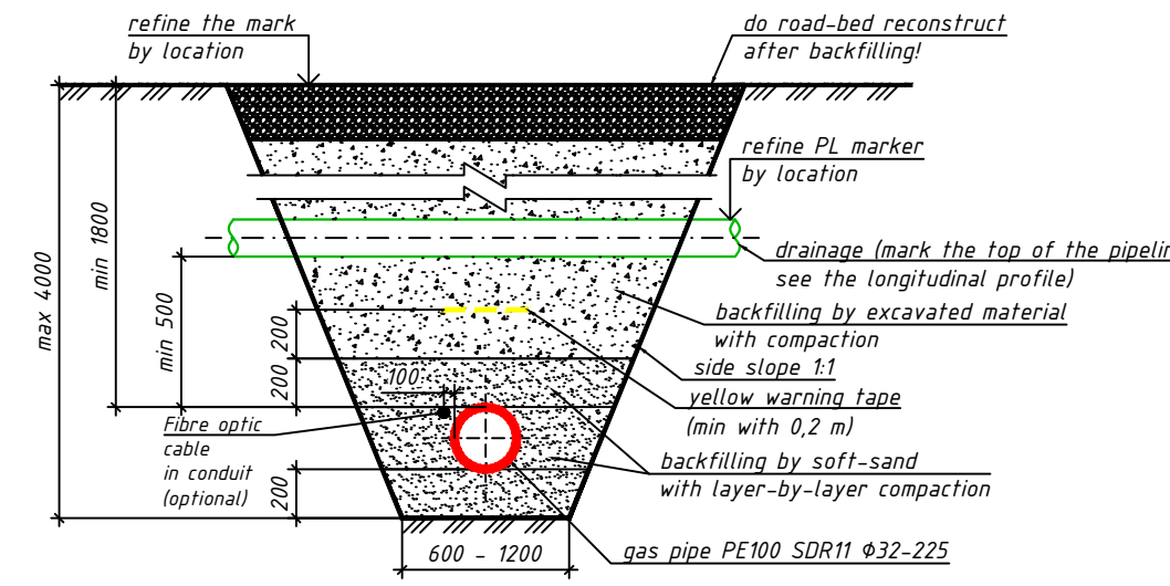
Gas pipe crossing drainage pipe under it
