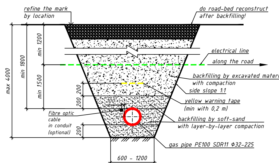
Gas pipe crossing electrical line that goes along the road
