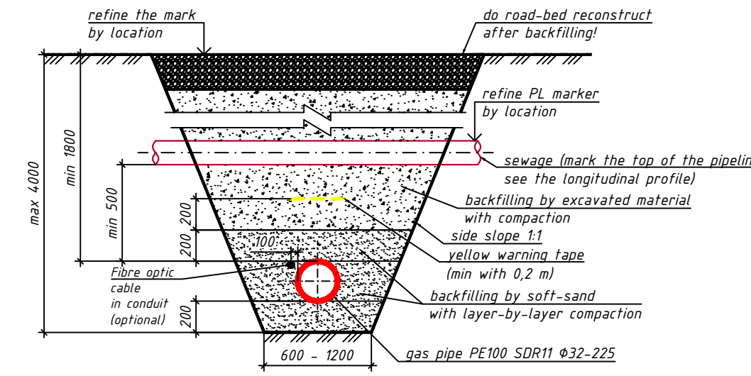
Gas pipe crossing sewage pipe under it
