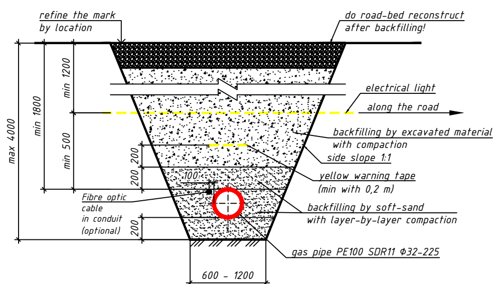
Gas pipe crossing electrical light that goes along the road
