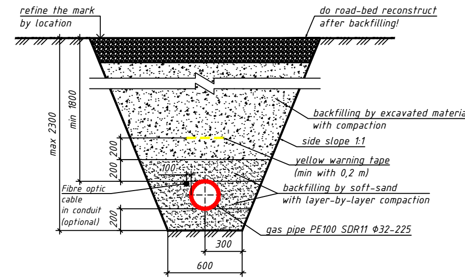
Without crossing communications (trench depth max 2300 mm)
