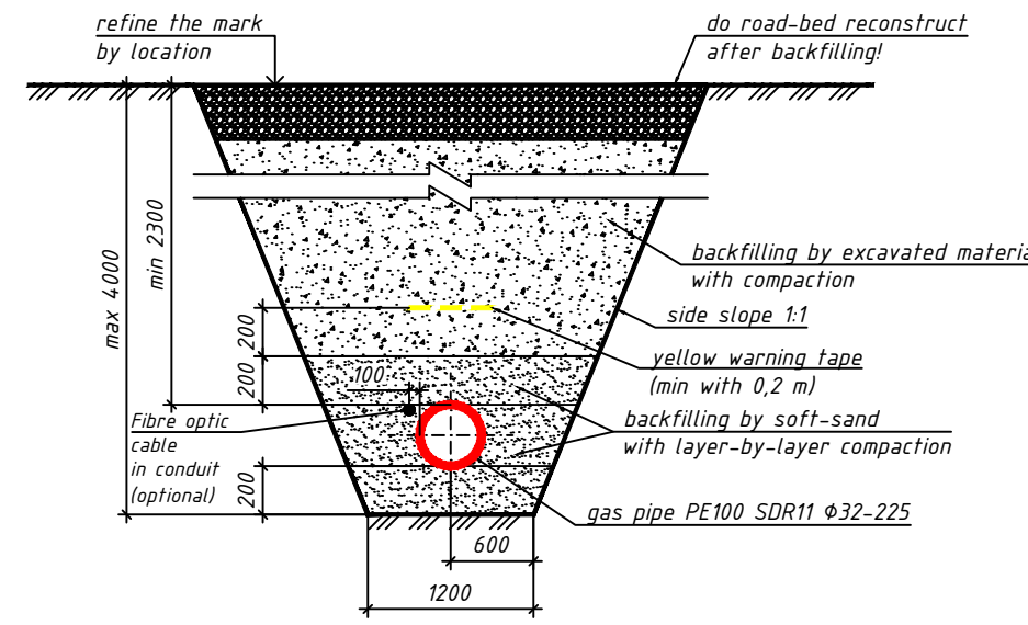
Without crossing communications (trench depth max 4000 mm)
