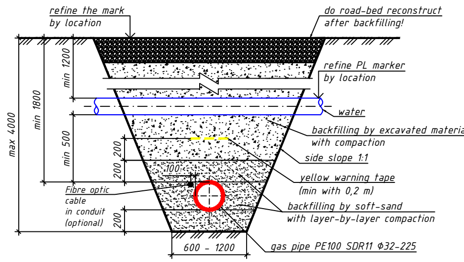
Gas pipe crossing water pipe under it
