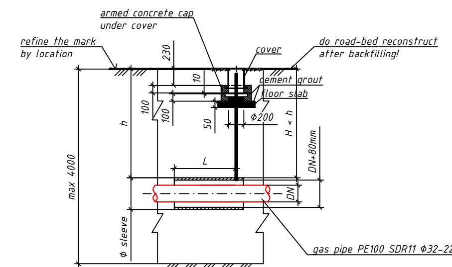
Covering control tube
