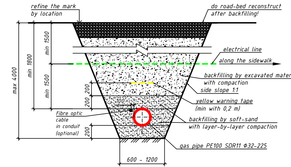
Gas pipe crossing electrical line that goes along the sidewalk
