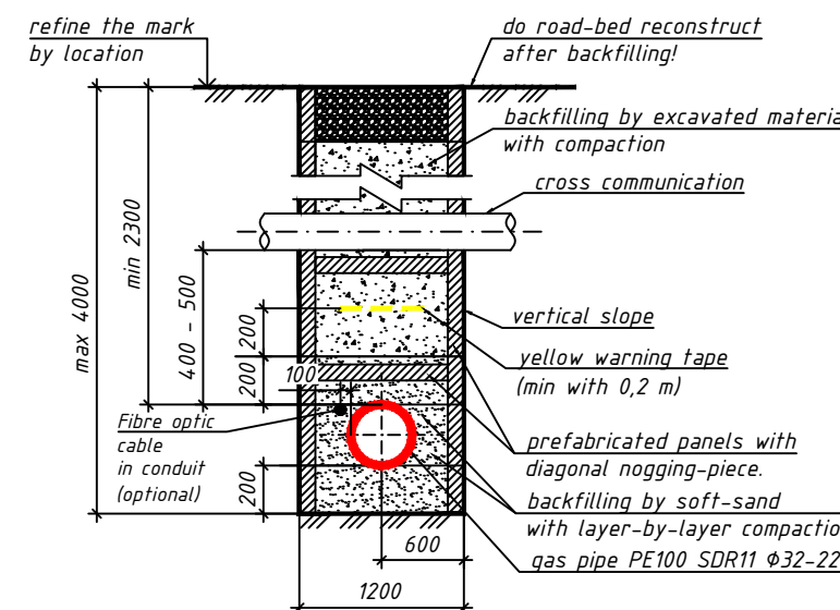
Trench with vertical slopes and prefabricated panels
