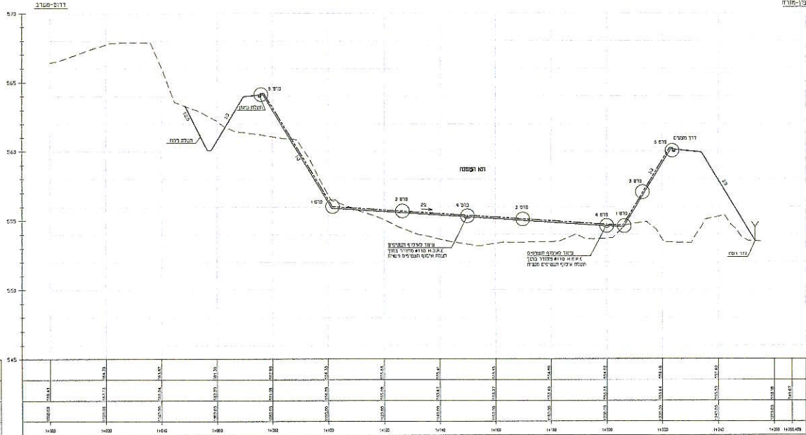
Scale 1:500/100 ROAD NAME sec 1-1 [sec 1-1]
